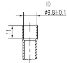
吸气管详细 SUCTION TUBE
